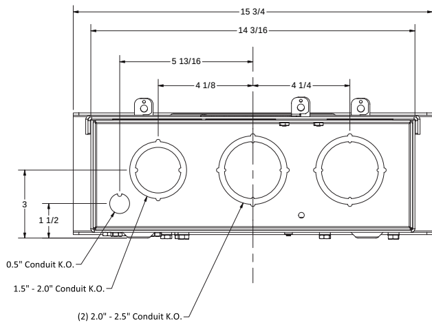
Figure 1, MSB200L Overhead
