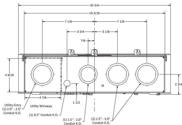
Figure 3, MSB200L & MSB200H Underground
