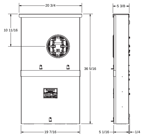
Figure 4, MSB200L & MSB200H Underground
