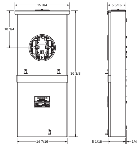
Figure 2, MSB200L Overhead
