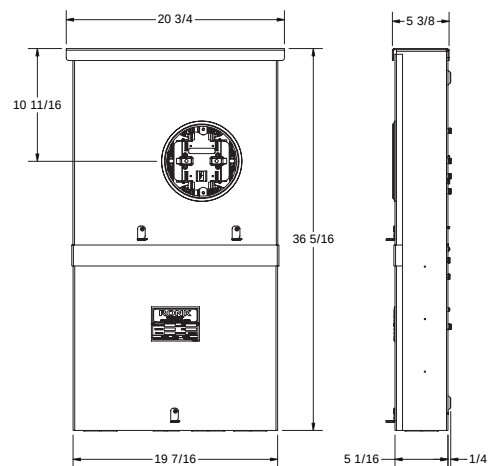
Figure 4, MSB Meter Socket Underground
