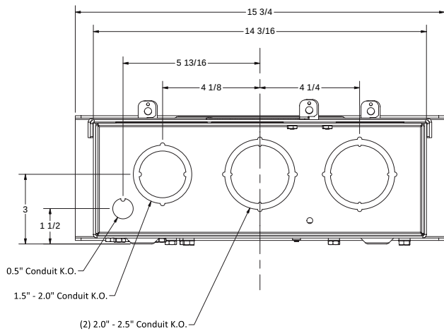
Figure 1, MSB Meter Socket Overhead
