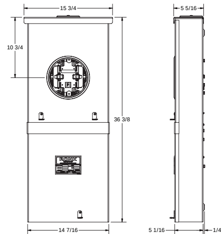
Figure 2, MSB Meter Socket Overhead
