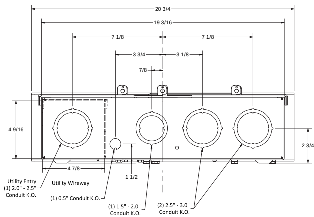
Figure 3, MSB Meter Socket Underground
